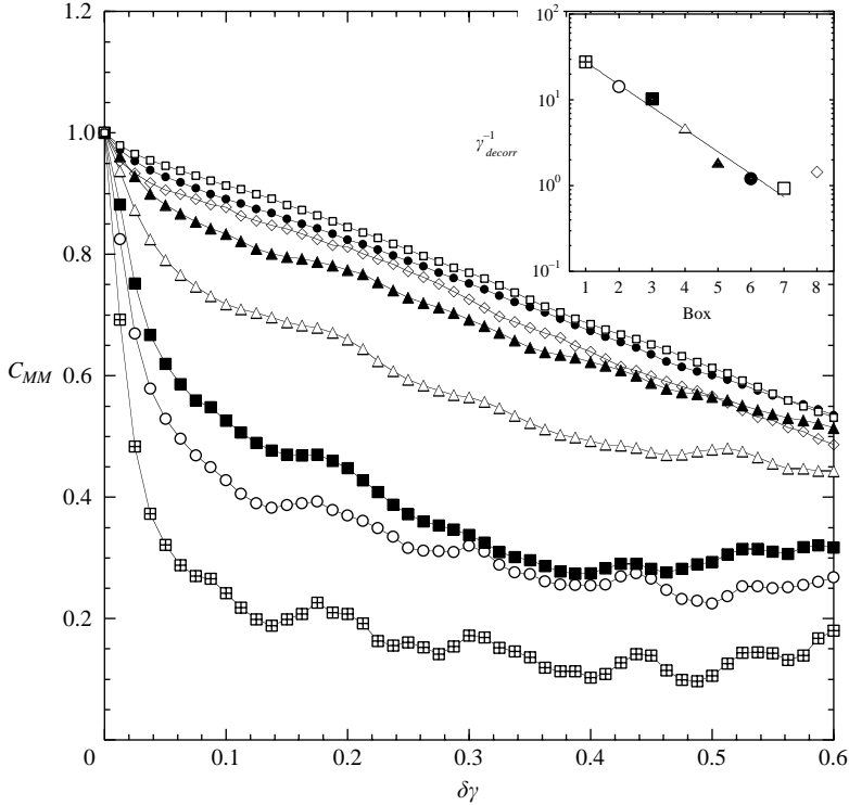
FIGURE 12. Run 2 (stationary flow): autocorrelation C_{M_r\theta M_r\theta} of the cross-component M_{r\theta} . \boxplus , box 1; \circ , box 2; \blacksquare , box 3; \triangle , box 4; \blacktriangle , box 5; \bullet , box 6; \square , box 7; \diamond , box 8. Inset: initial decorrelation rate \gamma_{decorr}^{-1} for each box, (4.6).
