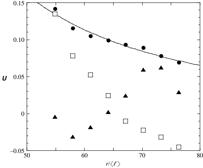
FIGURE 7. Run 2 (stationary flow): tensor \mathbf{U} versus box number. The components of \mathbf{U} ( \blacktriangle , U_{rr} ; \square , U_{\theta\theta} ; \bullet , U_{r\theta} ) are derived from the data in figure 6 through (3.15), using the value M_0 = 1.0 \text{ mm}^2 (see § 3.3.2). The solid line is a best fit of U_{r\theta} to a function cst/r^2 .
